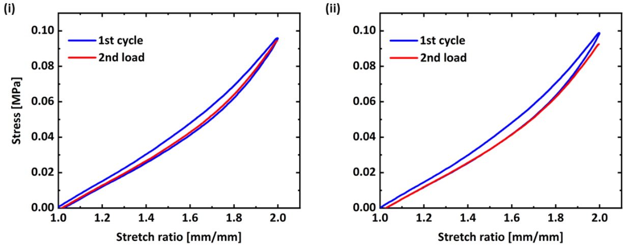
Fig. S2 Cyclic tests of HAp/DN gels ( n = 5 ) with different waiting time during the cyclic test. Blue line is first load-unload curve, and red line is second load curve after waiting from first load-unload for (i) 0 min, (ii) 30 min. The second loading curve almost overlaps with the first unloading curve, indicating no self- recovery. From these results, the contribution of energy dissipation E_p due to the interfacial debonding between polymer chain and HAp crystal is negligible.
